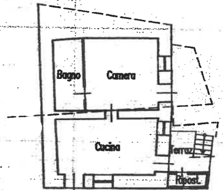
PIANO TERRA h=255
